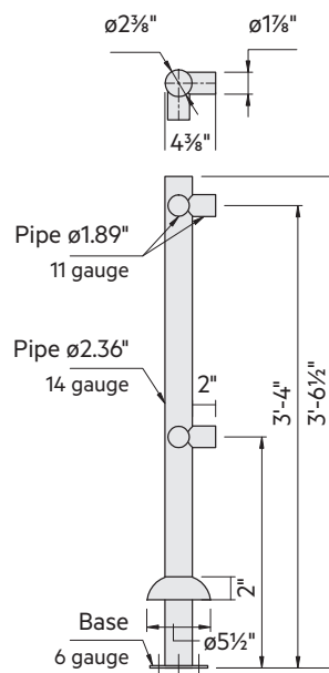
Vertical Corner Post BG-GR-CP-SS
