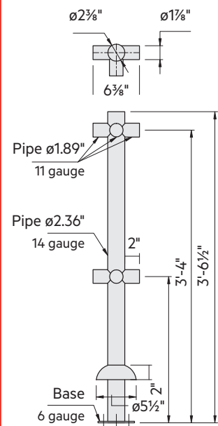
Vertical Post Three Way BG-GR-TP-SS
