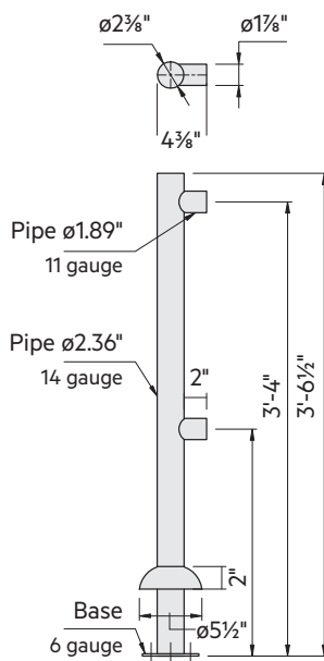
Vertical Post One Way BG-GR-EP-SS
