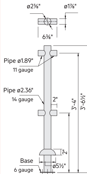
Vertical Post Two Way BG-GR-MP-SS
